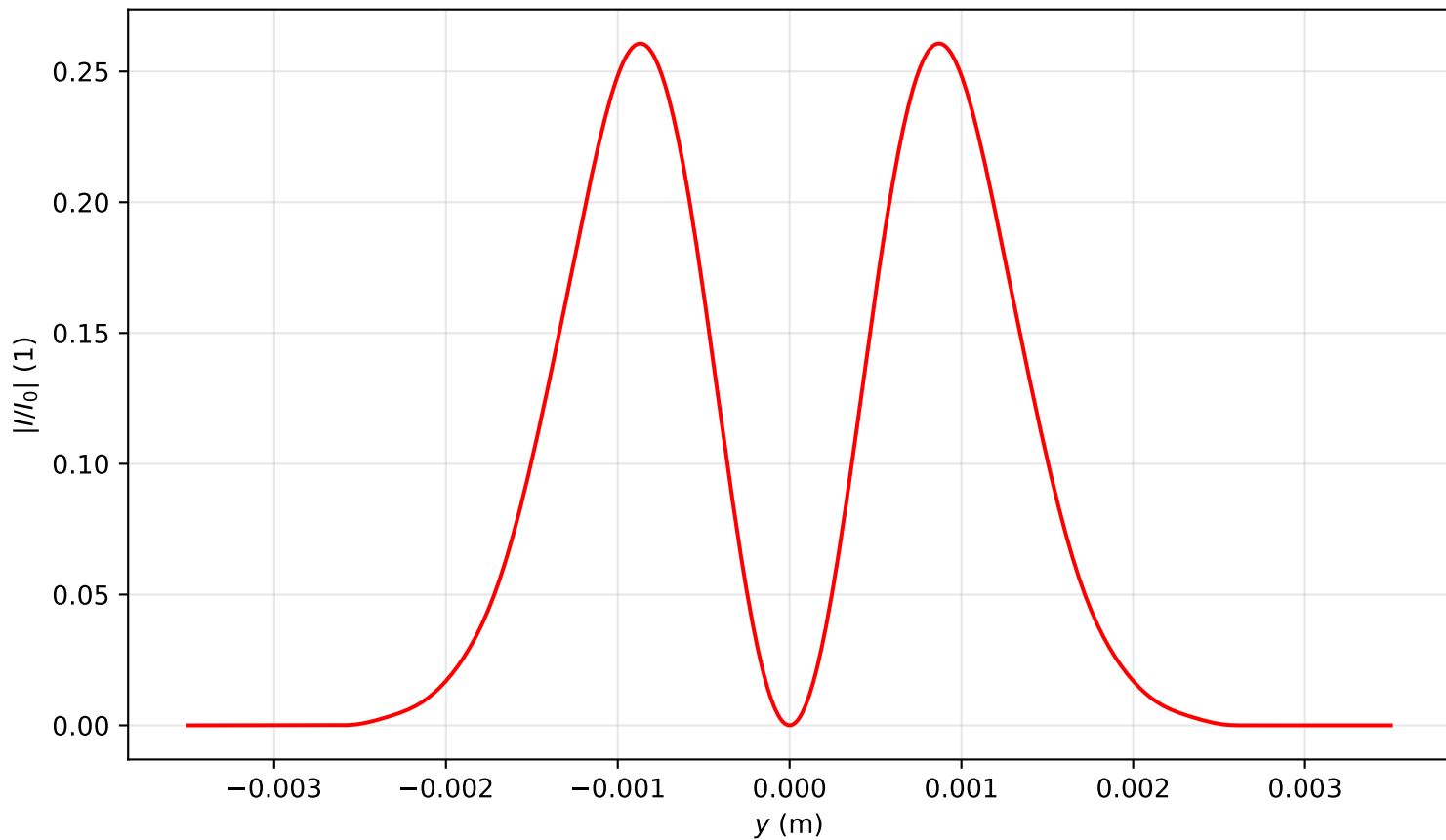
Intensity profile I(x=0, y, z=2.946)/I_0 , P_{in}=0.5P_{cr} , artificial time
